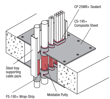
Concrete Floor
