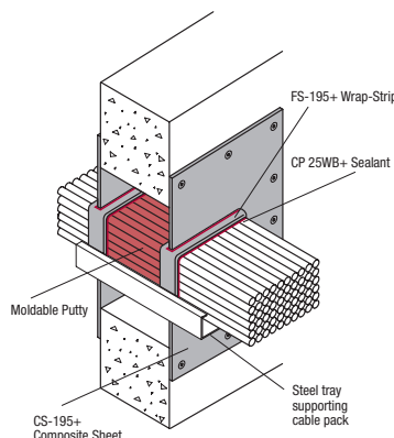
Solid Masonry, Hollow Masonry or Concrete Wall
