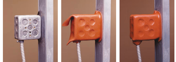
Electrical box being firestopped.
